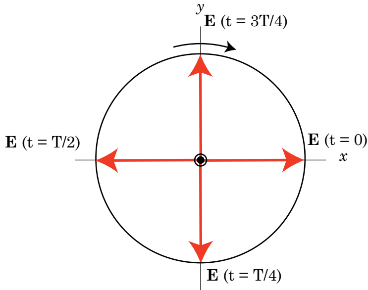
Left hand circular polarization. The direction of the electric vector at 0, 1/4, 1/2, and 3/4 periods, T . The z -axis points out of the page.
